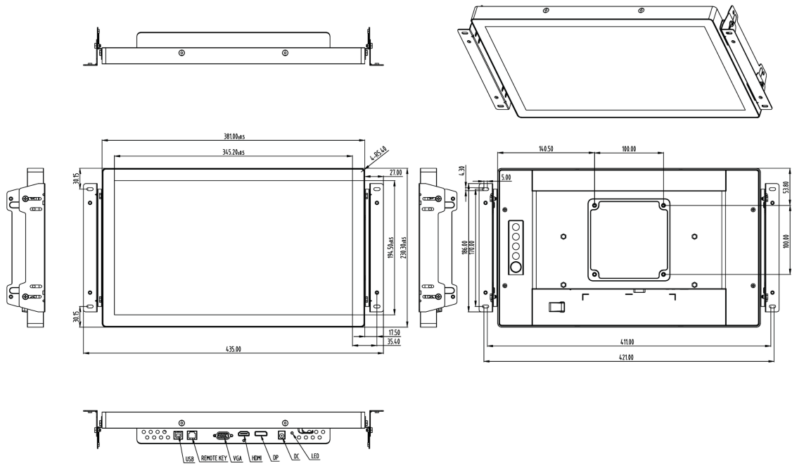
ProLite TF1634MC-B8X with brackets
